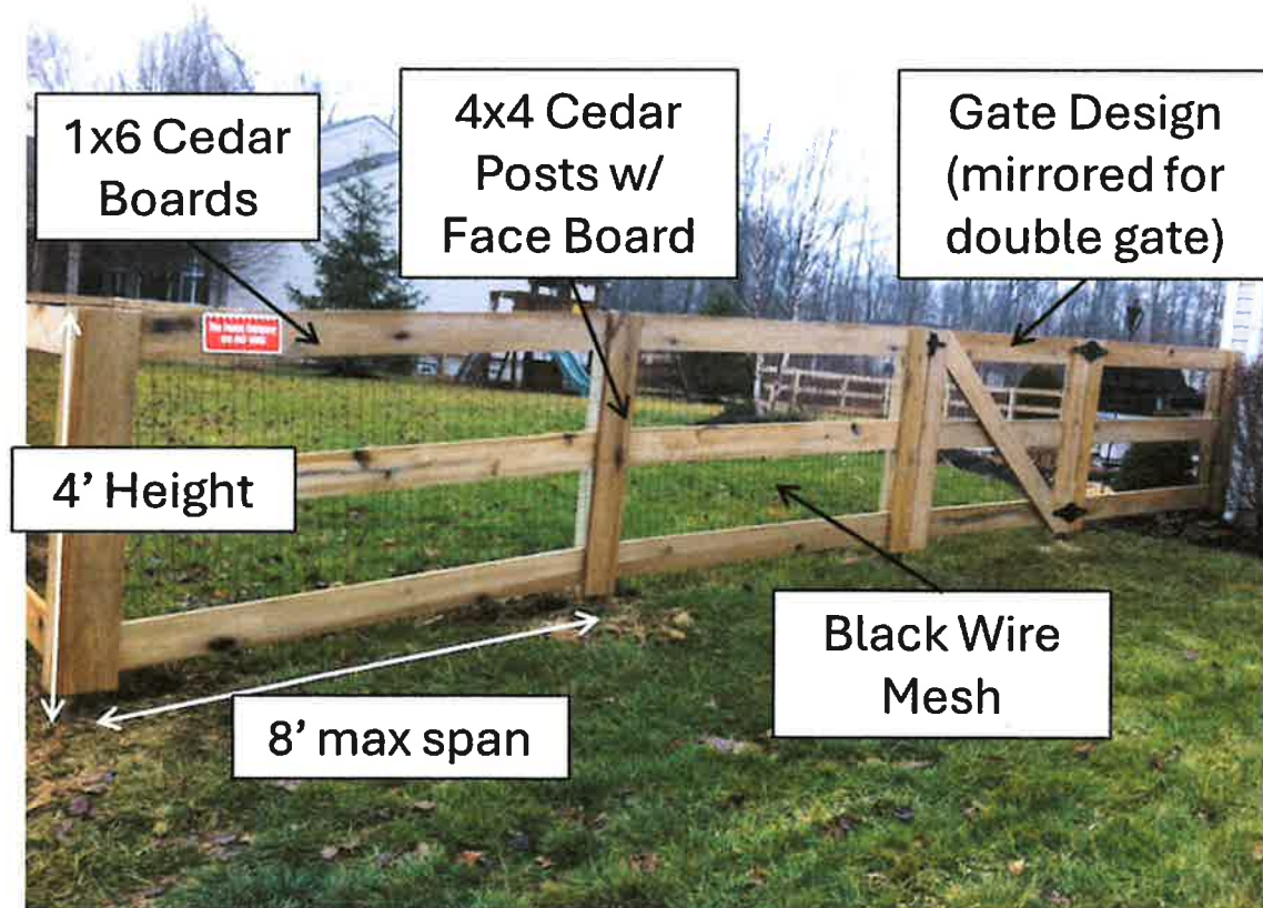
Figure 2: Fence Design Details (Cedar Post and Rail w/ Face Boards and Black Wire Mesh)
