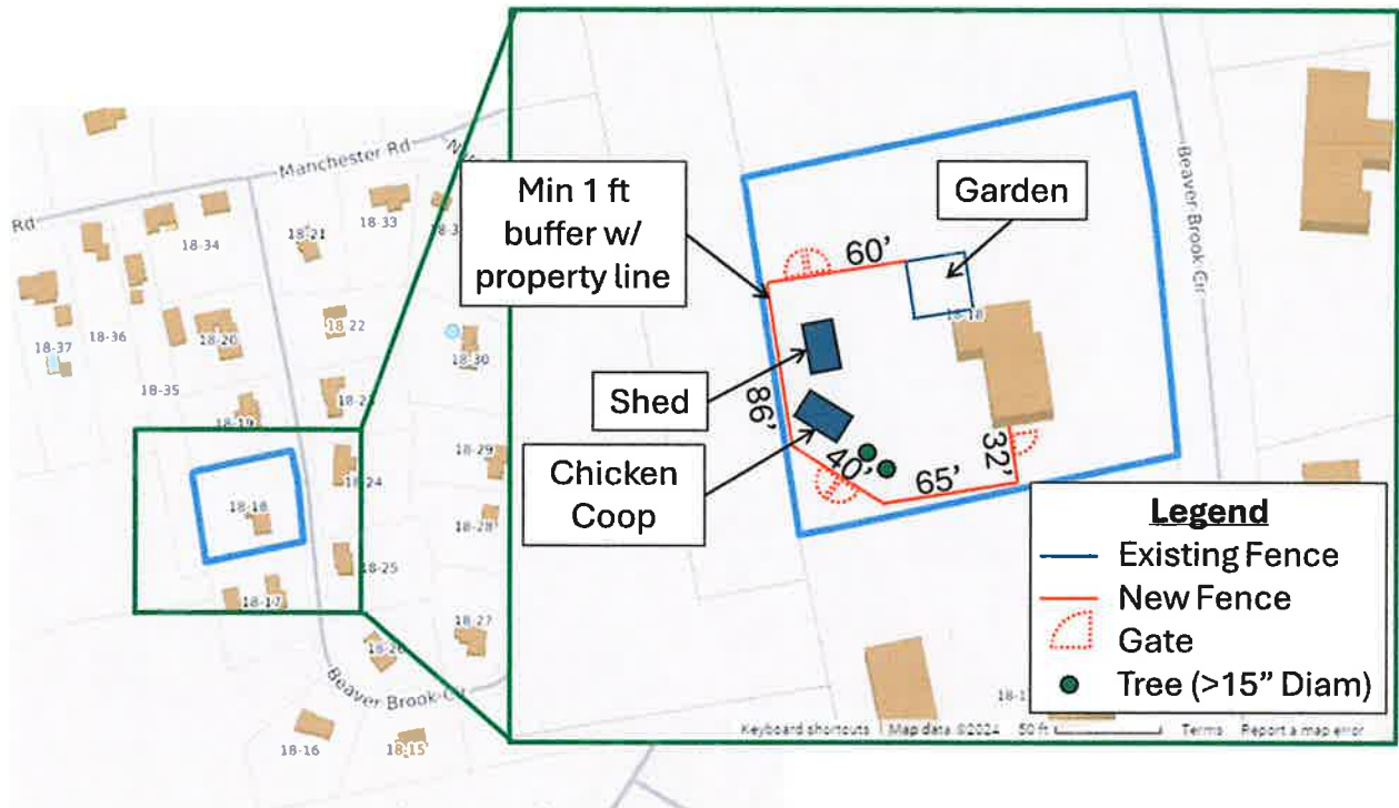
Figure 1: Installation Plan and Dimensions
